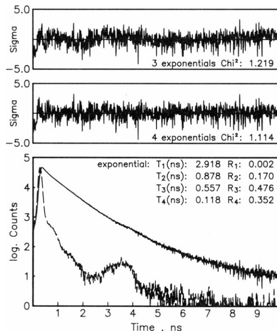
FIGURE 2 Conventional decay analysis at a single wavelength ( \lambda_{\text{em}} = 685 nm) for a light II-adapted sample (same data as in Figs. 1 and 4). The residual plots and \chi^2 value are given for a three- and a four-exponential model function (top). The lower part of the Fig. shows the semilogarithmic presentation of the fluorescence decay (solid line) and the excitation function (dashed line).
